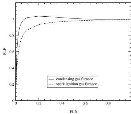
Figure 2: PLC for condensing & spark ignition furnaces.
