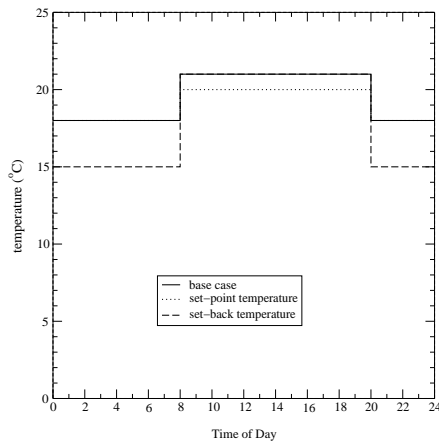
Figure 6: Set-back & set-point control strategies
