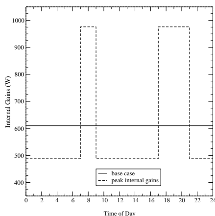
Figure 8: Constant and peak internal gain profiles
