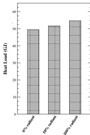
Figure 4: Radiant heat injection into main zone.
