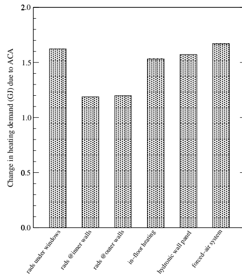
Figure 5: Impact of ACA on annual heating loads
