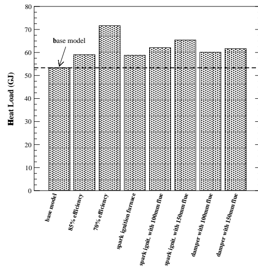
Figure 3: Sensitivity to HVAC parameters.
