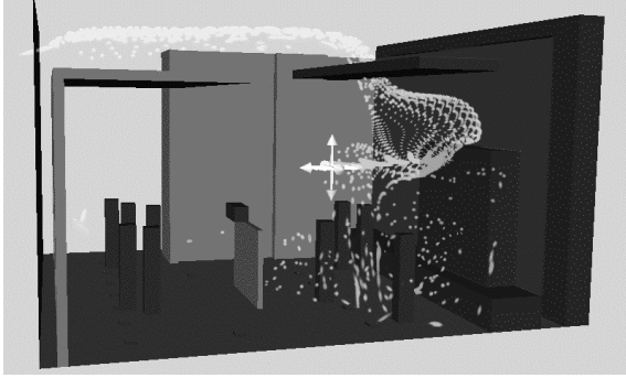
Figure 3: CFD model of gallery (view from side)
