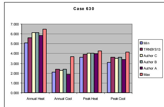
Figure 4: East / West Shaded Window Orientations
